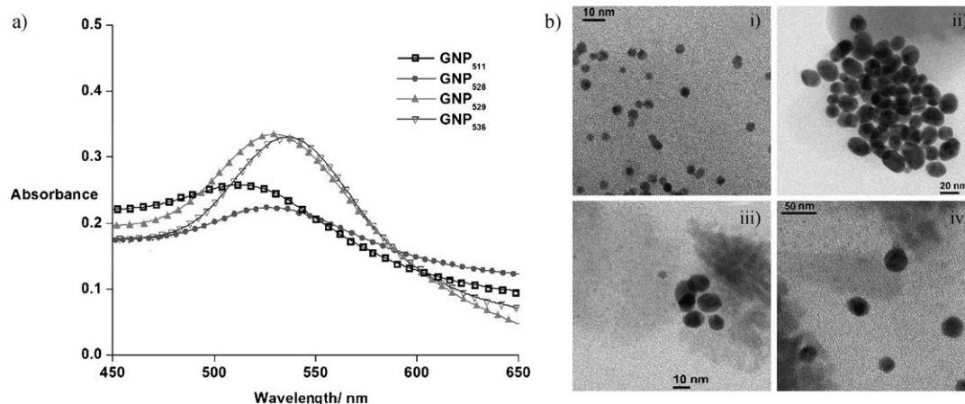
Figure 1. a) SPR peaks of GNPs of varying sizes: GNP 511 , GNP 528 , GNP 529 , and GNP 536 . b) TEM images of i) GNP 511 , ii) GNP 528 , iii) GNP 529 , and iv) GNP 536 .
