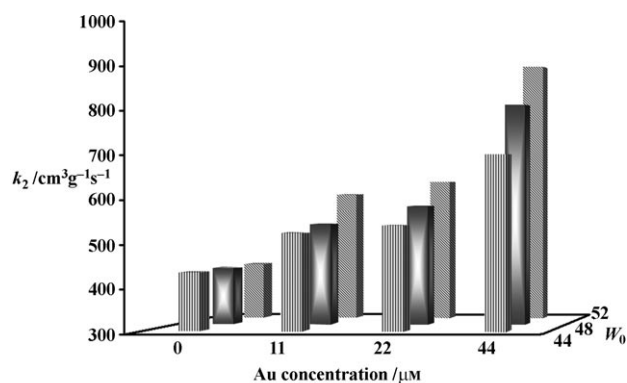
Figure 2. Variation of the second-order rate constant k_2 for the lipase-catalyzed hydrolysis of p -nitrophenyl n -octanoate in GNP-doped CTAB reverse micelles with varying W_0 values and GNP concentrations at z=4.8 and 25^\circ\text{C} . [CTAB] = 50 \text{ mM} , [enzyme] = 1.02 \times 10^{-6} \text{ g mL}^{-1} , [substrate] = 3 \text{ mM} . Experimental errors are within \pm 1\text{--}2\% .
