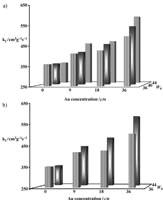
Figure 3. Variation of the second-order rate constant k_2 for the lipase-catalyzed hydrolysis of p -nitrophenyl n -octanoate in GNP-doped CTAB reverse micelles with varying W_0 values and GNP concentrations at z=6.4 (a) and 8.0 (b) and 25^\circ\text{C} . [CTAB] = 50 \text{ mM} , [enzyme] = 1.02 \times 10^{-6} \text{ g mL}^{-1} , [substrate] = 3 \text{ mM} . Experimental errors are within \pm 1\text{--}2\% .
