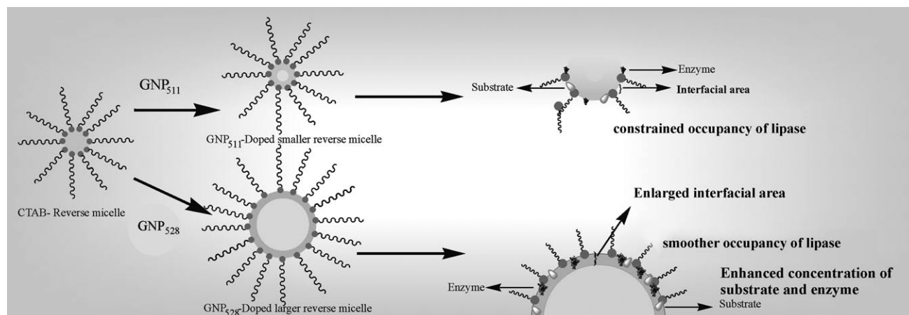
Scheme 1. Pictorial representation of lipase in GNP-doped reverse micelles.
