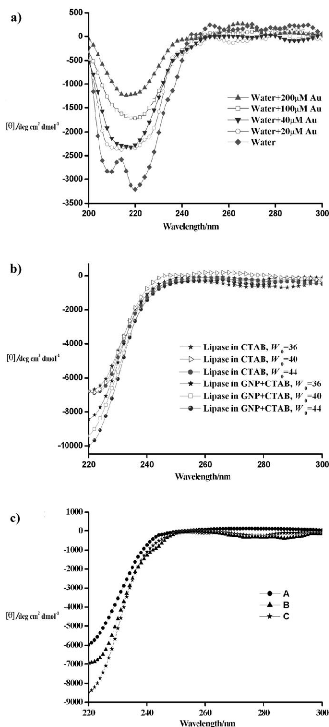
Figure 4. a) CD spectra of CV lipase in water with varying concentrations of GNPs. b) CD spectra of lipase in 50 mM CTAB reverse micelles in the absence of GNPs and in GNP-doped reverse micelles with varying W_0 values. c) CD spectra of CV lipase in CTAB reverse micelles at W_0=40 and z=6.4 with the GNP/lipase premixed solution (A), without GNPs (B), and with \text{GNP}_{528} -doped reverse micelles (C).
